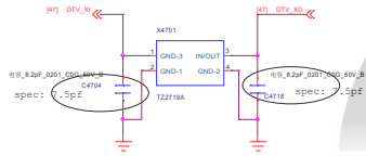
26MHz crystal
